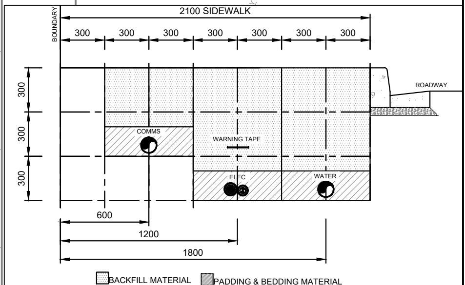
TYPICAL SERVICE TRENCH DETAIL
