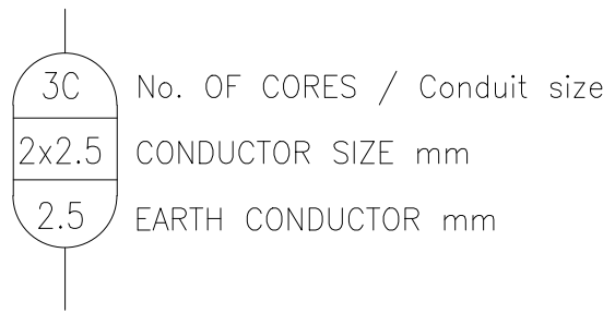
CABLE INDICATOR DETAIL
