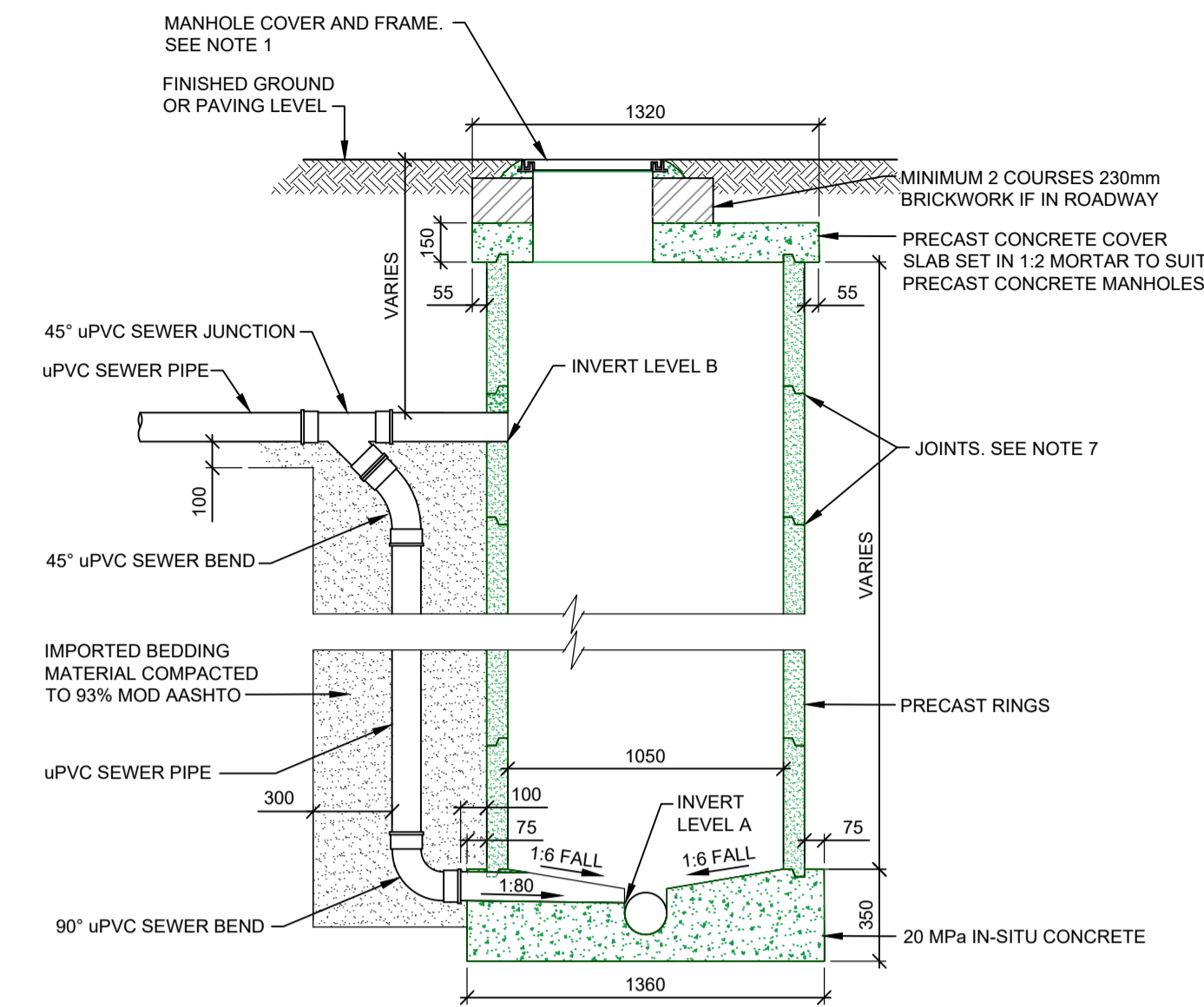
SECTION THROUGH TYPICAL SEWER MANHOLE WITH BACKDROP INLET SCALE 1 : 25
