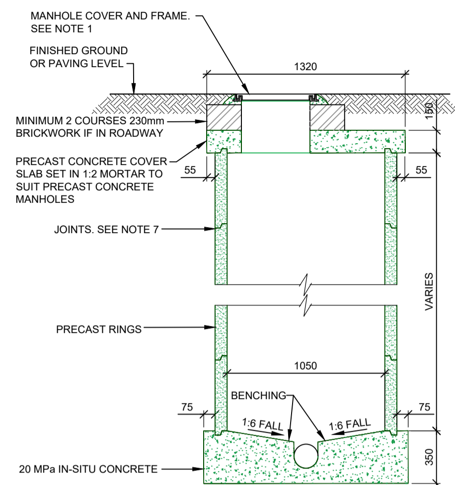
SECTION THROUGH TYPICAL SEWER MANHOLE SCALE 1 : 25
