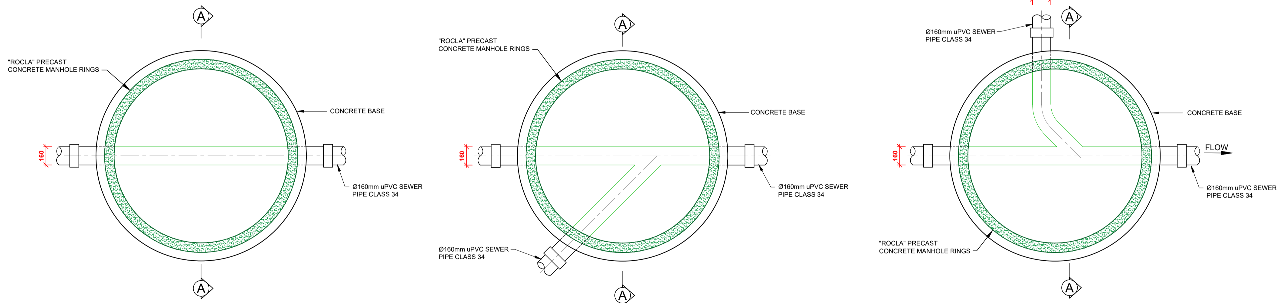
TYPICAL MANHOLE LAYOUTS SCALE 1 : 20
